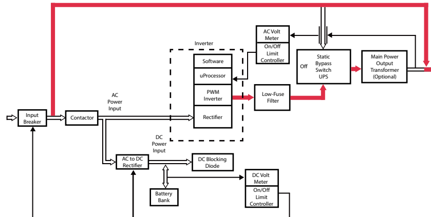
Figure 4 Single Line Drawings –External Maintenance Bypass Operation
