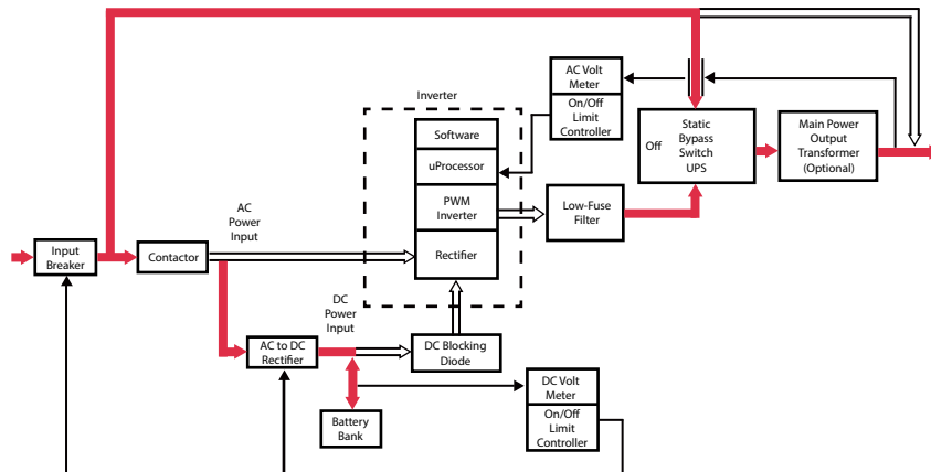
Figure 2 Single Line Drawing - Static Bypass Operation
