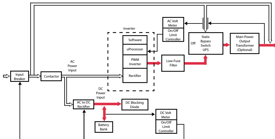
Figure 3 Single Line Drawings -AC Loss/Battery Operation
